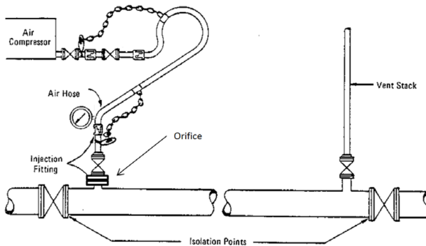
Figure 6. Direct Method with Orifice and pressure gauge relocated closer to orifice. (Direct Purging)
