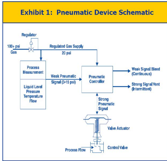
Figure 4: Pneumatic Device Schematic 61
