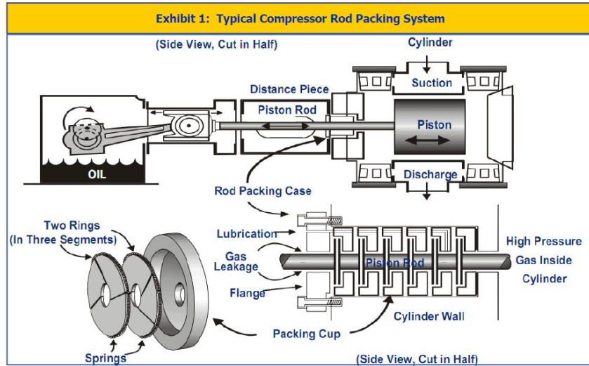
Figure 6: Typical Compressor Rod Packing System 2
