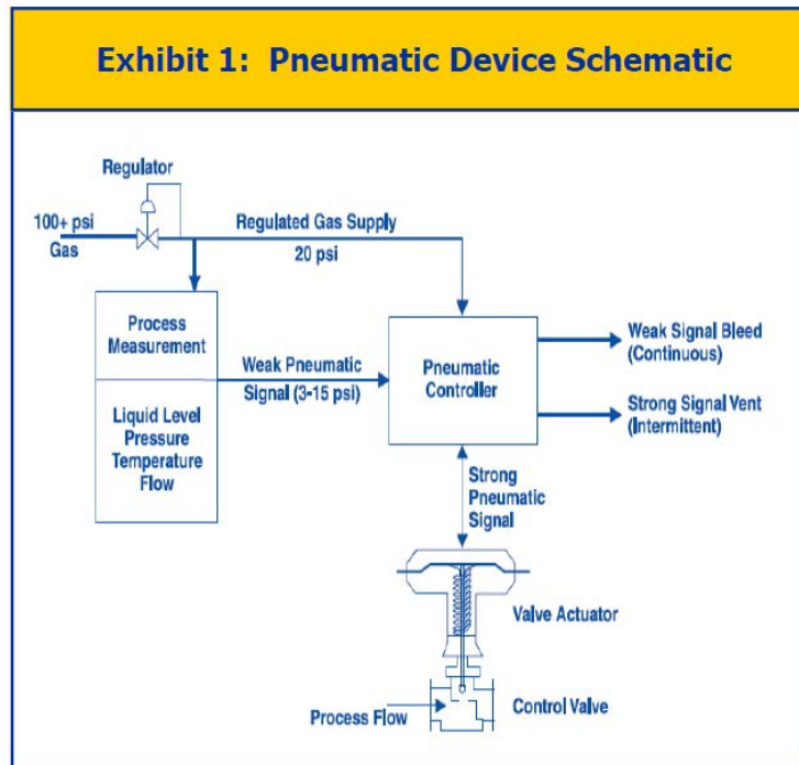
Figure 2: Pneumatic Device Schematic 61
